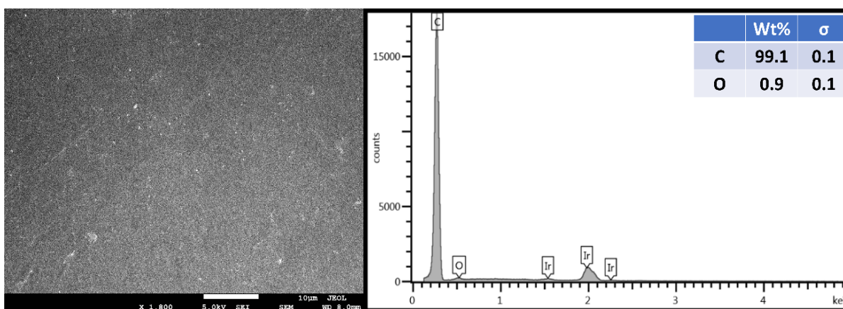
Figure 3: Side view (surface) of PP compounded with 5 wt.% Mg(OH)_2 .
