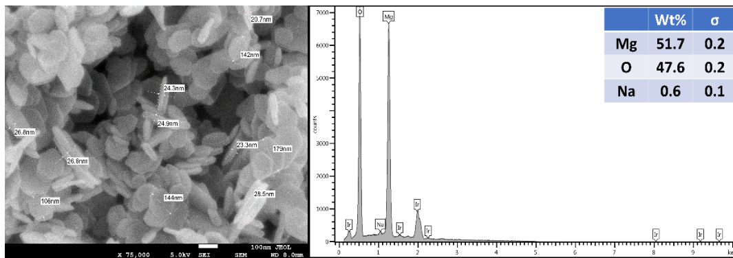
Figure 1: SEM image and EDX spectrum of the Mg(OH)_2 crystals.
