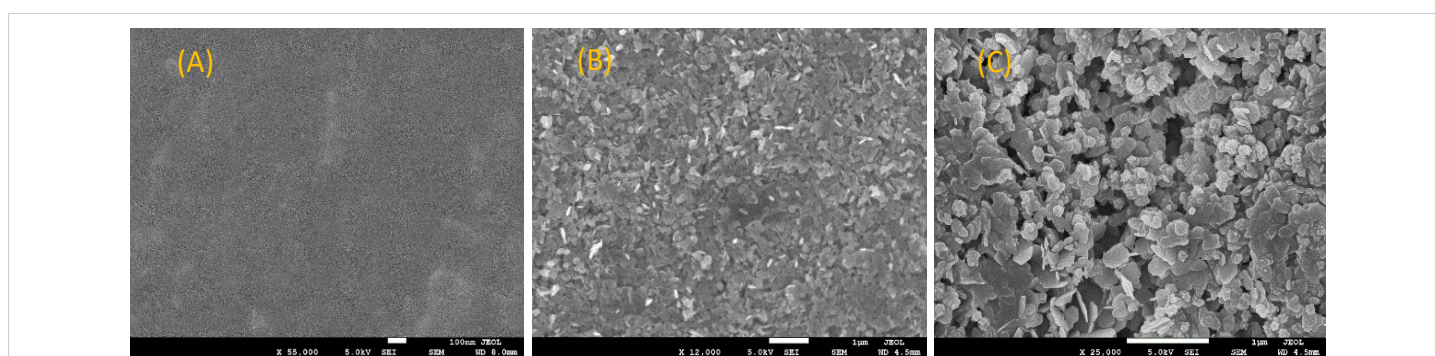
Figure 5: SEM images of (A) neat PP, (B) PP that was thermally embossed with Mg(OH) 2 NPs, and (C) PP that was thermally embossed with Cu-infused Mg(OH) 2 NPs.
