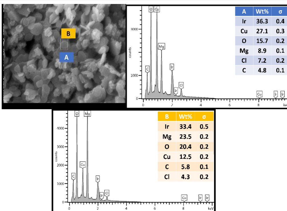
Figure 2: SEM image and EDX spectrum of the Cu-infused Mg(OH)_2 crystals.
