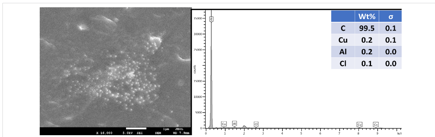
Figure 4: Side view (surface) of PP compounded with 5 wt.% Cu-infused Mg(OH) 2 .
